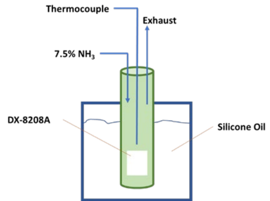
7.5% NH 3 gas exposure set-up
